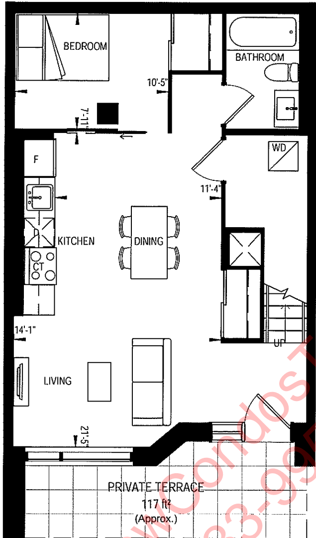
LEVEL 1
