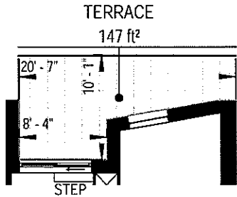
LEVEL: 7
